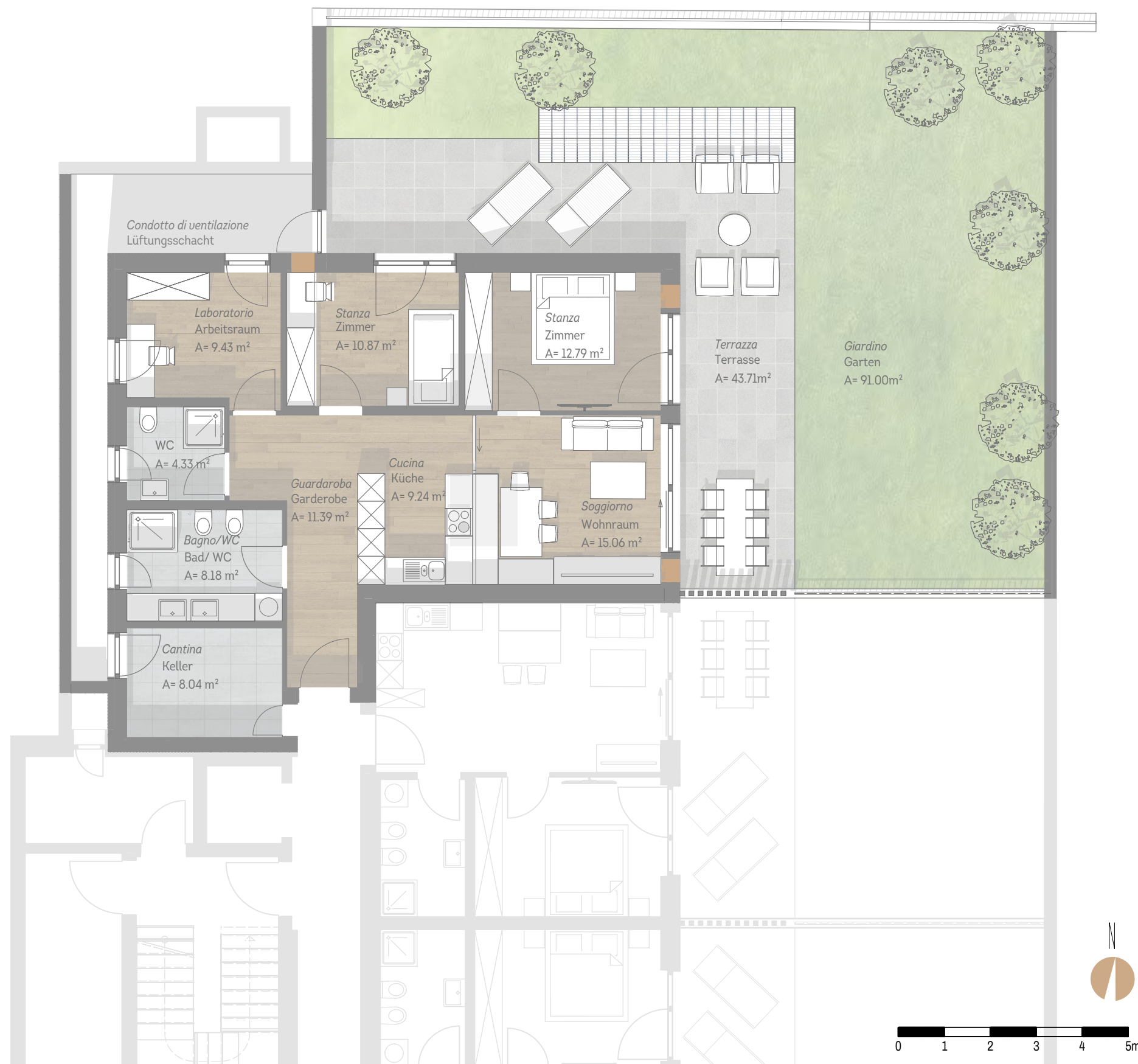
Erdgeschoss - Piano terra
