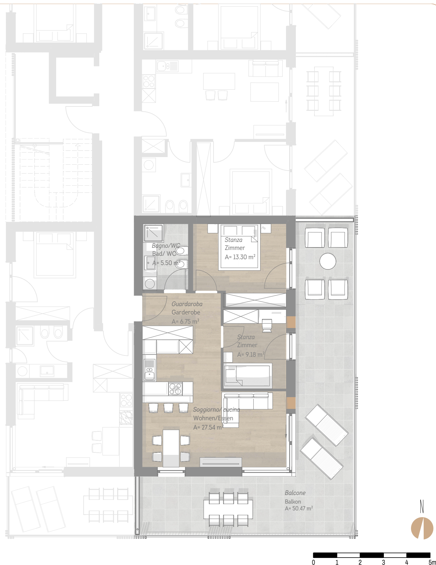
2. Obergeschoss - Secondo piano
