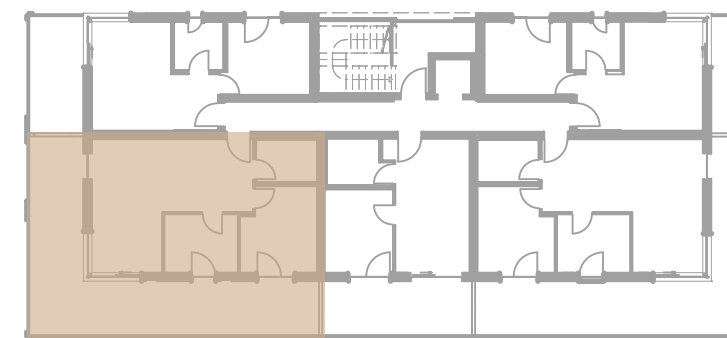
2. Obergeschoss - Secondo piano
